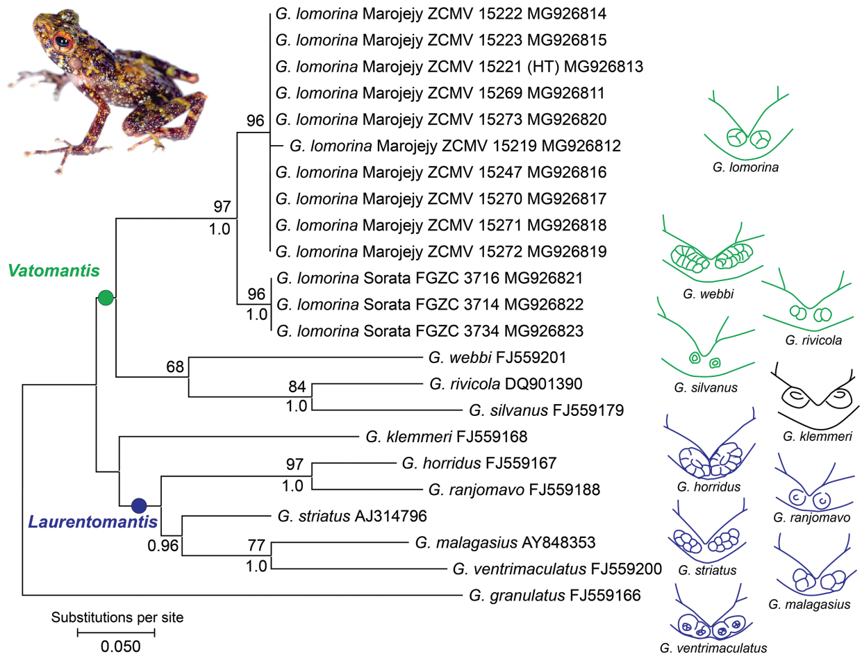
Figure 1. Preliminary phylogenetic tree of Gephyromantis ( Vatomantis ) lomorina sp. n., based on Maximum Likelihood analysis of a 532 bp fragment of the mitochondrial 16S rRNA gene. Numbers at nodes indicate bootstrap values in percent (500 replicates, above) and posterior probabilities from a Bayesian Inference analysis (20 million generations, below), shown only if >50 % (bootstrap) or >90 % (posterior probabilities). Each specimen/species is followed by the corresponding GenBank accession number used in the alignment. Schematic drawings of femoral glands of all species in the subgenera Laurentomantis and Vatomantis as well as of G. klemmeri are shown to the right of the phylogeny, and coloured according to the subgenus to which they are assigned.
